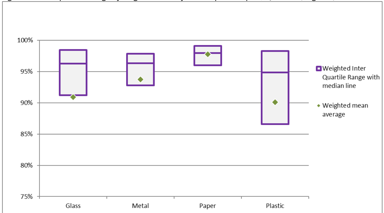
Figure 7: Inter-quartile range of target material from output samples, Q1 2019 (England)
