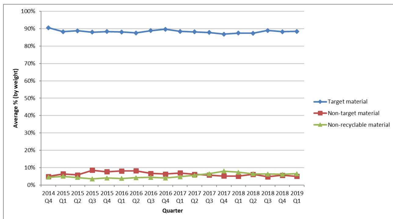
Figure 6: Fluctuations in input stream samples in Wales Q4 2014 – Q1 2019
