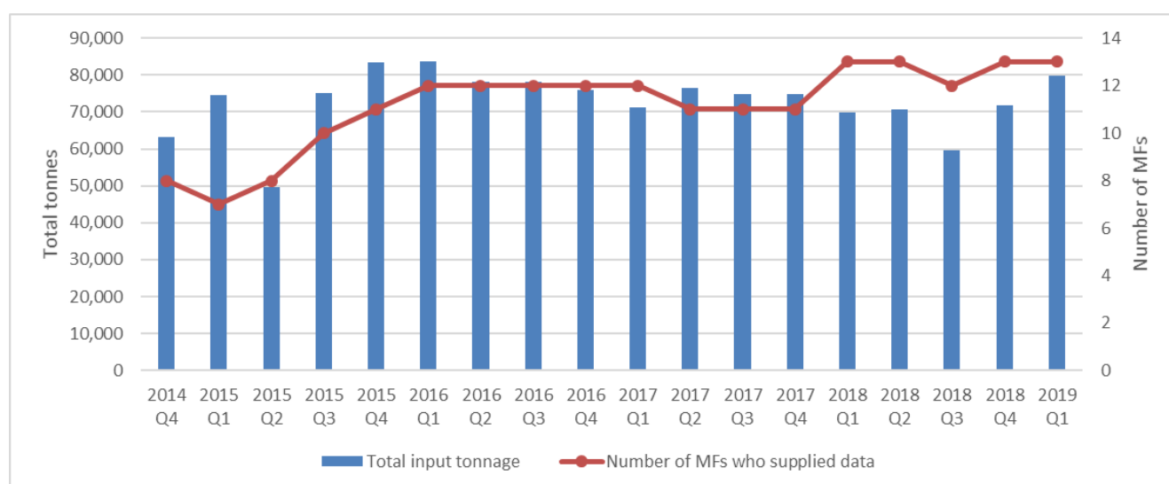
Figure 5 Changes in input tonnes in Wales Q4 2014 – Q1 2019
